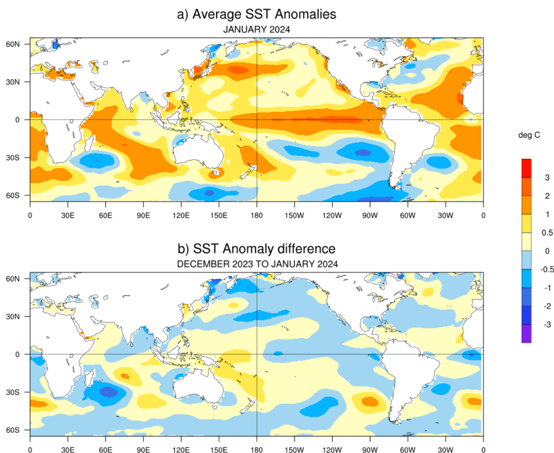
Fig.1: (a) Sea surface temperature (SST) anomalies ( o C) during January 2024 and (b) changes in the SST anomalies ( o C) from December 2023 to January 2024. SSTs were based on the ERSSTv5, NOAA, and anomalies were computed with respect to 30-year (1991-2020) long term mean.
