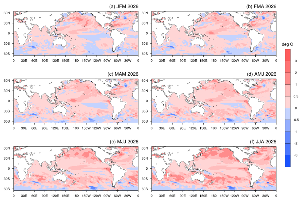
Fig.3: Forecasted Seasonal mean SST anomalies for three-monthly (a) January to March (JFM 2026), (b) February to April (FMA 2026), (c) March to May (MAM 2026), (d) April to Jun (AMJ 2026), (e) May to Jul (MJJ 2026) and (f) June to August (JJA 2026) Model bias correction base period: 1999-2008; Climatology base period:1991-2020).
