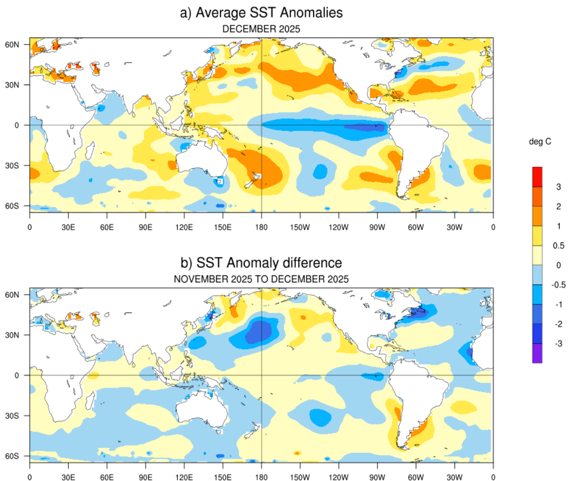
Fig.1: (a) Sea surface temperature (SST) anomalies (degC) during December 2025 and (b) changes in the SST anomalies (degC) from November 2025 to December 2025. SSTs are based on the ERSSTv5 (NCEP-NOAA), and anomalies are computed with respect to 30-year (1991-2020) long term mean.
