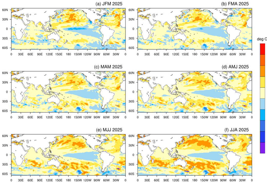
Fig.3: Forecasted Seasonal mean SST anomalies for three-monthly (a) January to March 2025 (JFM 2025), (b) February to April (FMA 2025) (c) March to May (MAM 2025), (d) April to June (AMJ 2025), (e) May to July (MJJ 2025) and (f) June to August (JJA 2025) (Model bias correction base period: 1999-2008; Climatology base period:1991-2020).
