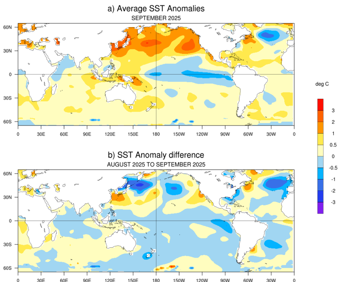
Fig.1: (a) Sea surface temperature (SST) anomalies (degC) during September 2025 and (b) changes in the SST anomalies (degC) from August 2025 to September 2025. SSTs are based on the ERSSTv5 (NCEP-NOAA), and anomalies are computed with respect to 30-year (1991-2020) long term mean.
