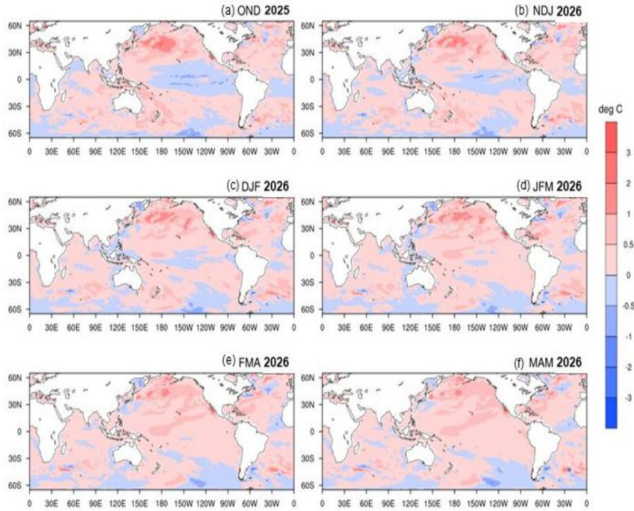
Fig.3: Forecasted Seasonal mean SST anomalies for three-monthly (a) October to December (OND 2025), (b) November to January (NDJ 2026), (c) December to February (DJF 2026), (d) January to March (JFM 2026), (e) February to April (FMA 2026) and (f) March to May (MAM 2026) Model bias correction base period: 1999-2008; Climatology base period:1991-2020).
